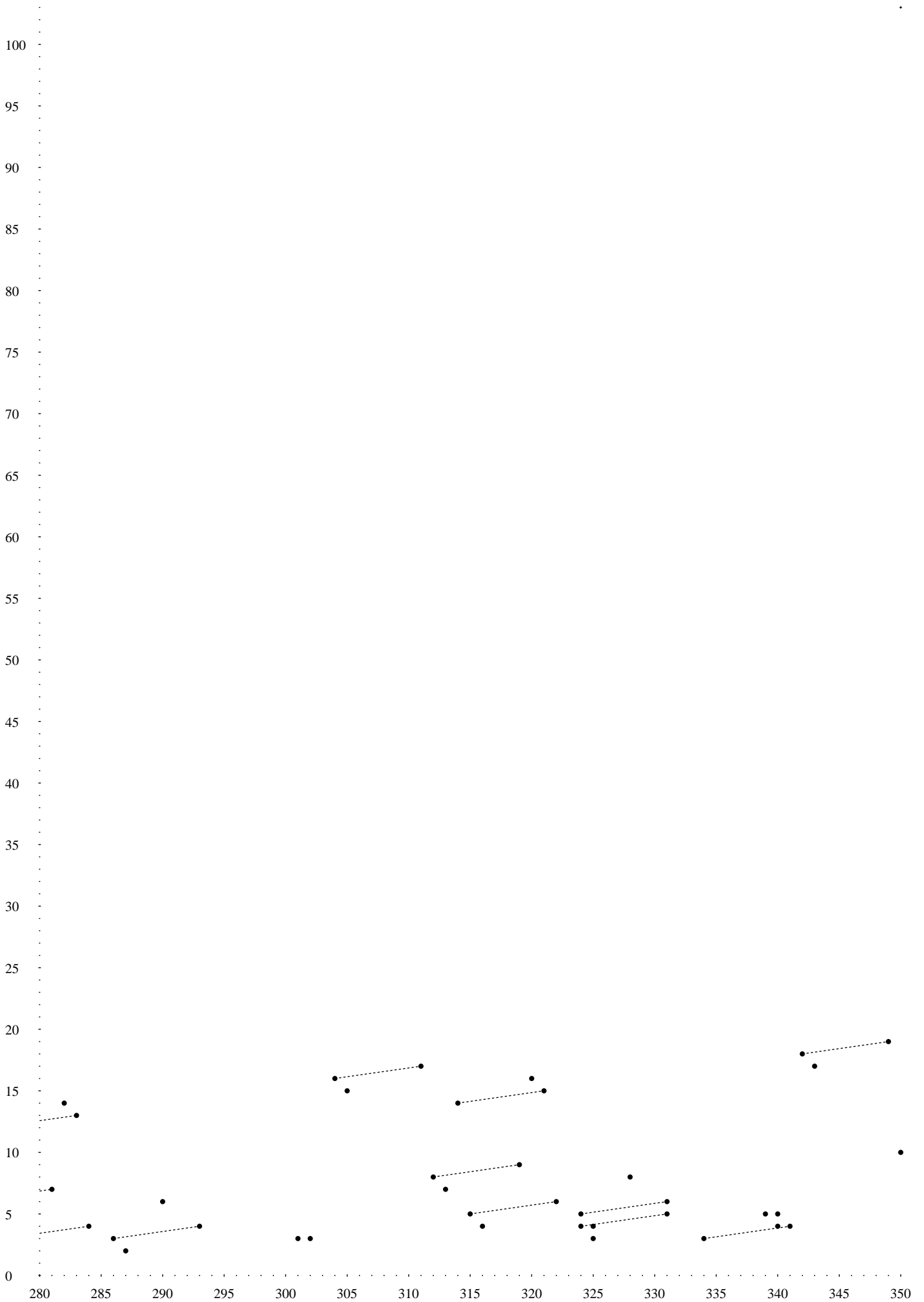
Toda complex S/(5, v_1, v_2)
